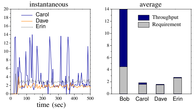
Fig. 7. Scenario 2: (\xi_C, \xi_E) = (1.7, 2.8) . Instantaneous and average throughput (Mb/s) are shown.
