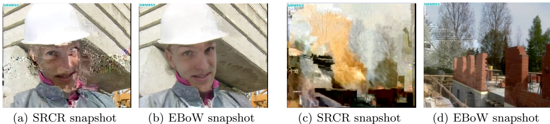
Fig. 2: foreman snapshots
