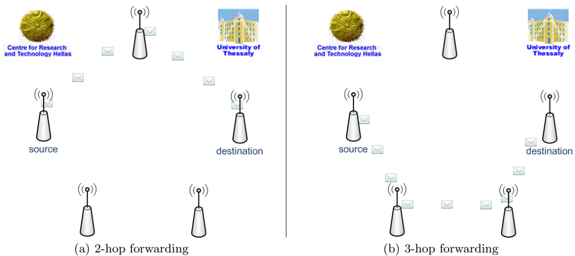
Fig. 3: GUI snapshots
