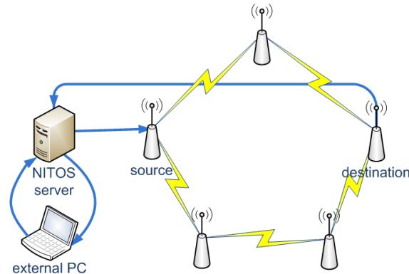
Fig. 1: Ring Network
