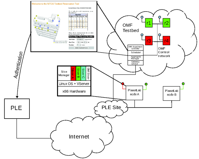
Fig. 1. OMF-PlanetLab integrated architecture.
