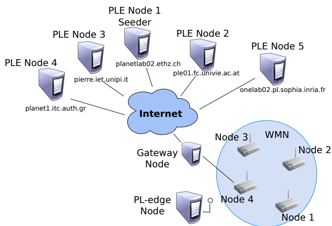
Fig. 2. Experiments setup.
