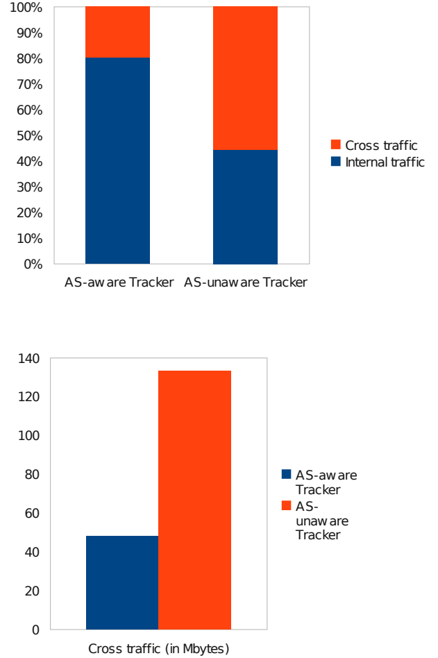
Fig. 3. Bittorrent optimization experiment results.
