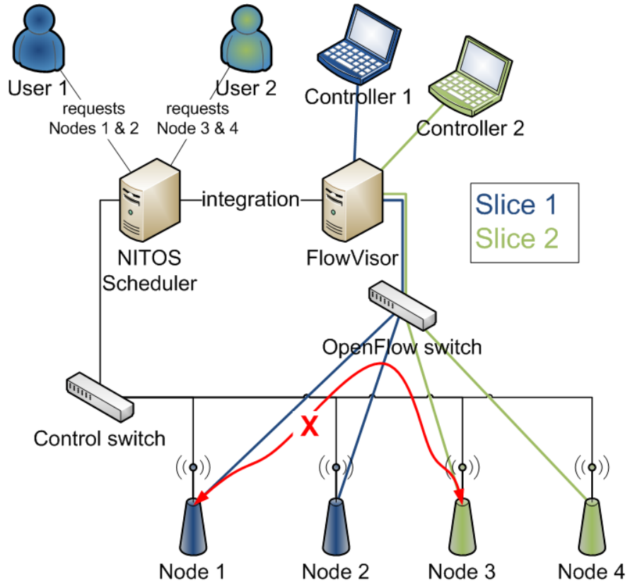
Fig. 1. NITOS Scheduler - FlowVisor integration
