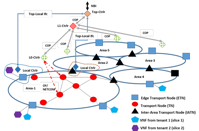
Fig. 1: Overview of the proposed transport network architecture and associated control plane hierarchy.
