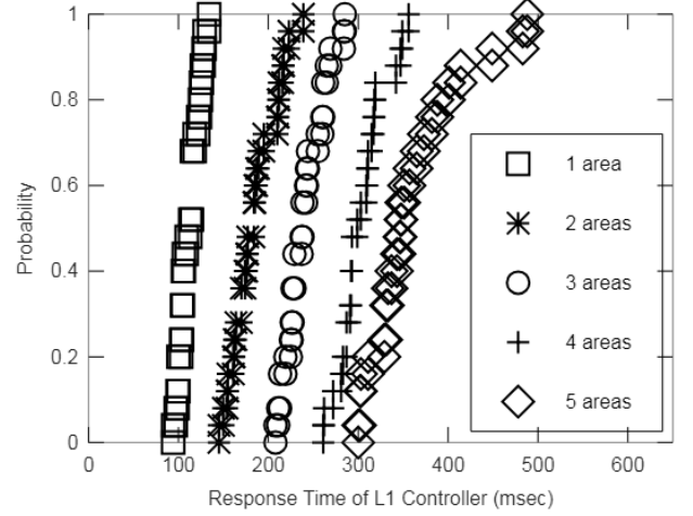
Fig. 5: Scaling of L1 controller response latency CDFs with increasing number of areas in provisioned path.
