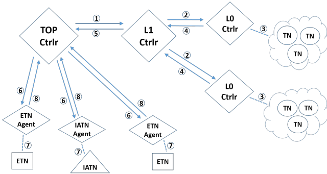
Fig. 3: Interactions among controllers for end to end path establishment.
