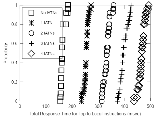
Fig. 6: Scaling of total response time of Local Agents of ETNs and IATNs in provisioned path.
