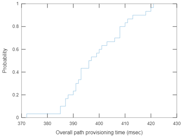
Fig. 7: CDF of overall delay for path provisioning in two-area experiment with areas and controllers distributed at two remote sites.
